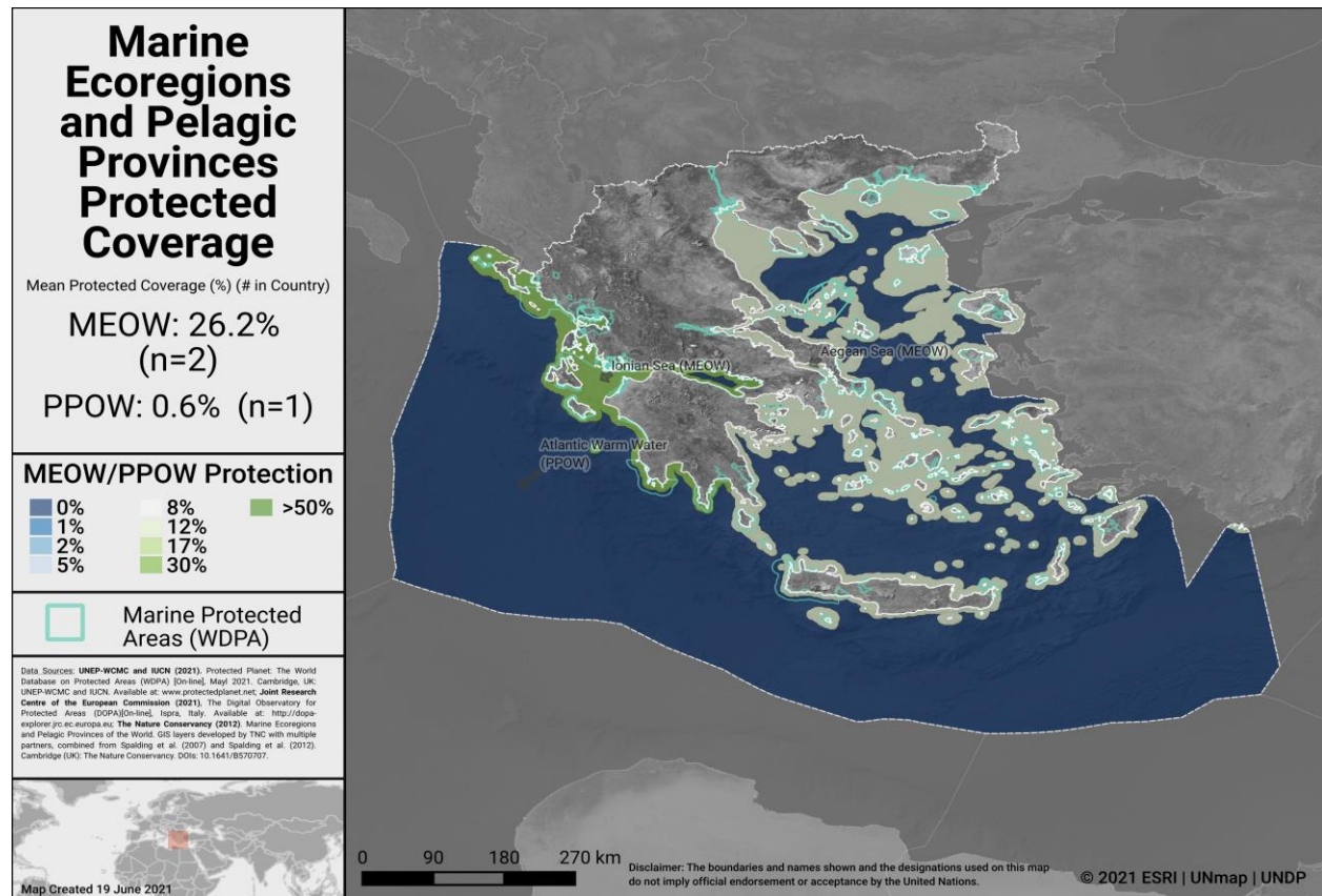
Marine ecoregions and pelagic provinces
