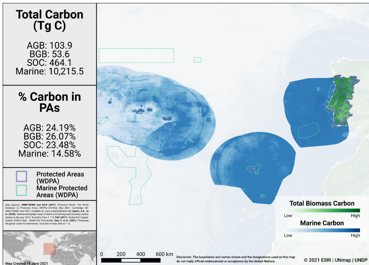
Carbon Stocks in Portugal
