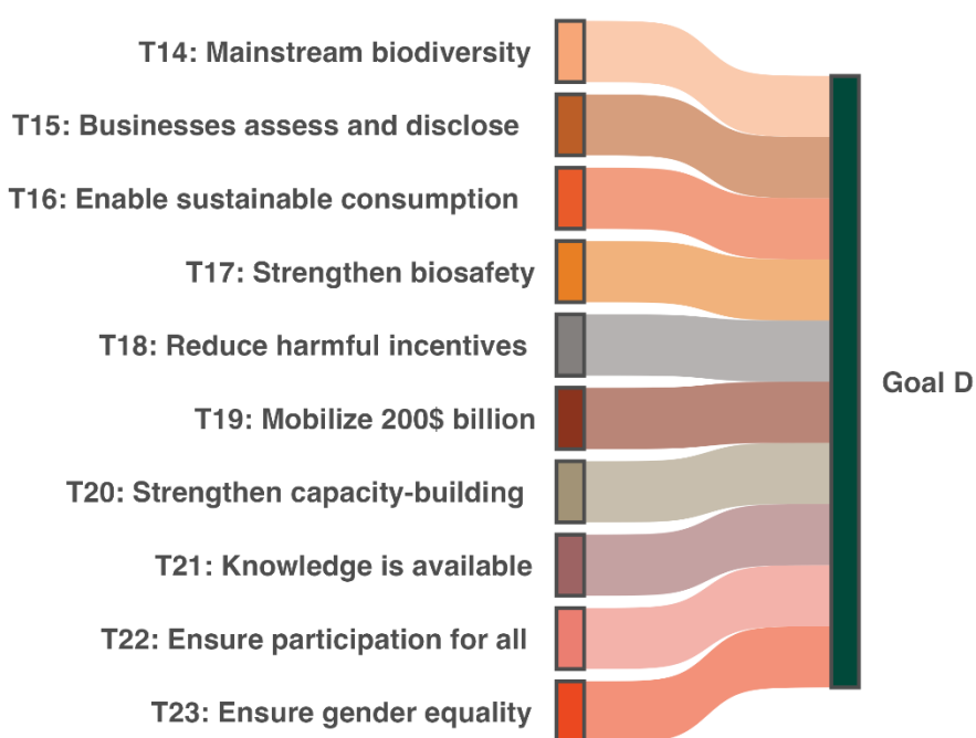
Figure 107 (II.C.D-LINKS) Framework targets associated with Goal D in Parties' national target submissions. A link is drawn between a target and the goal if at least one in three of all Parties' national targets from any UN group associated a target to the goal. Colours are used to highlight each target according to the official brand guidelines of the Framework and do not carry any additional meaning.
