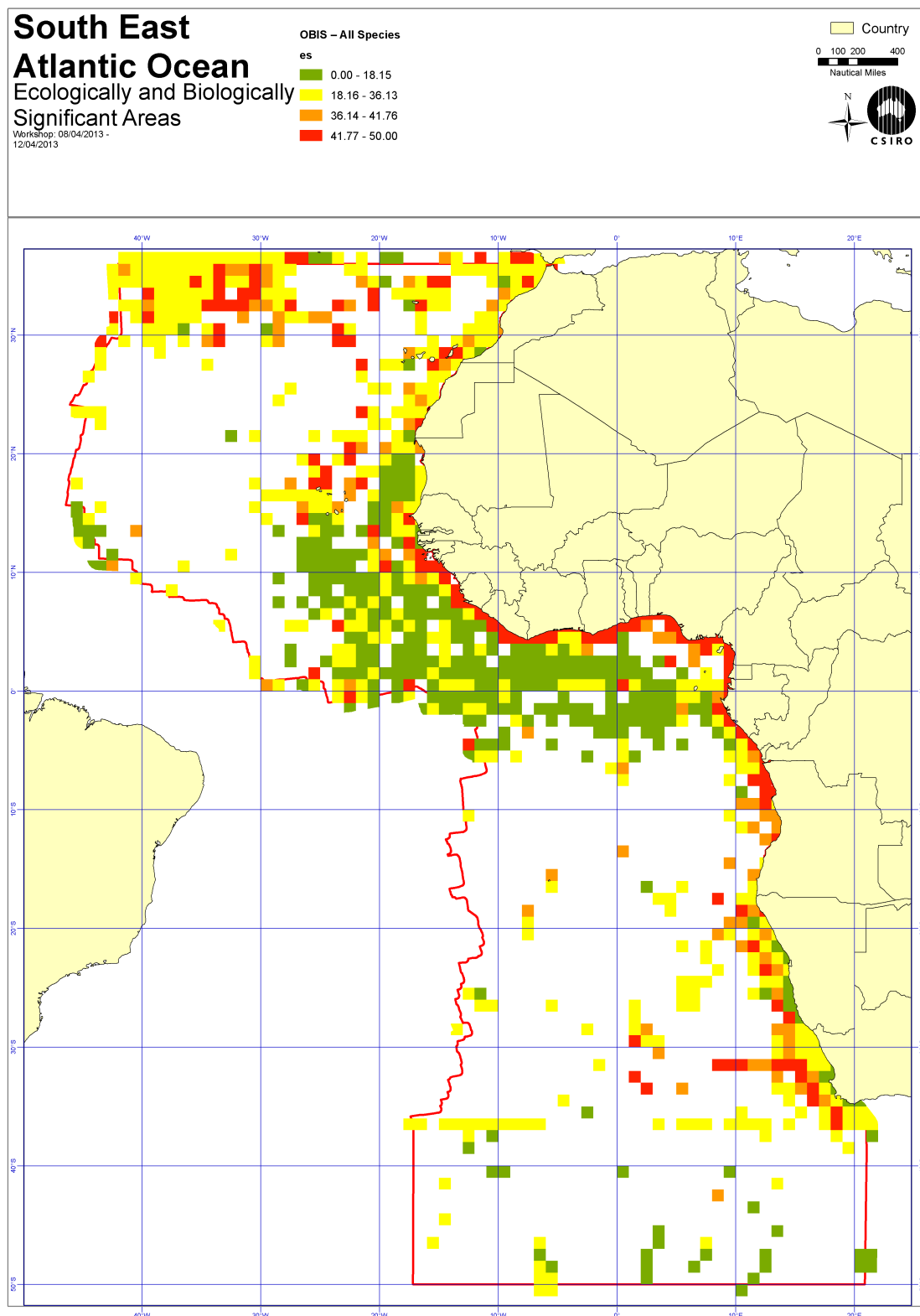
Figure 3.9: OBIS ES(50) for all species
