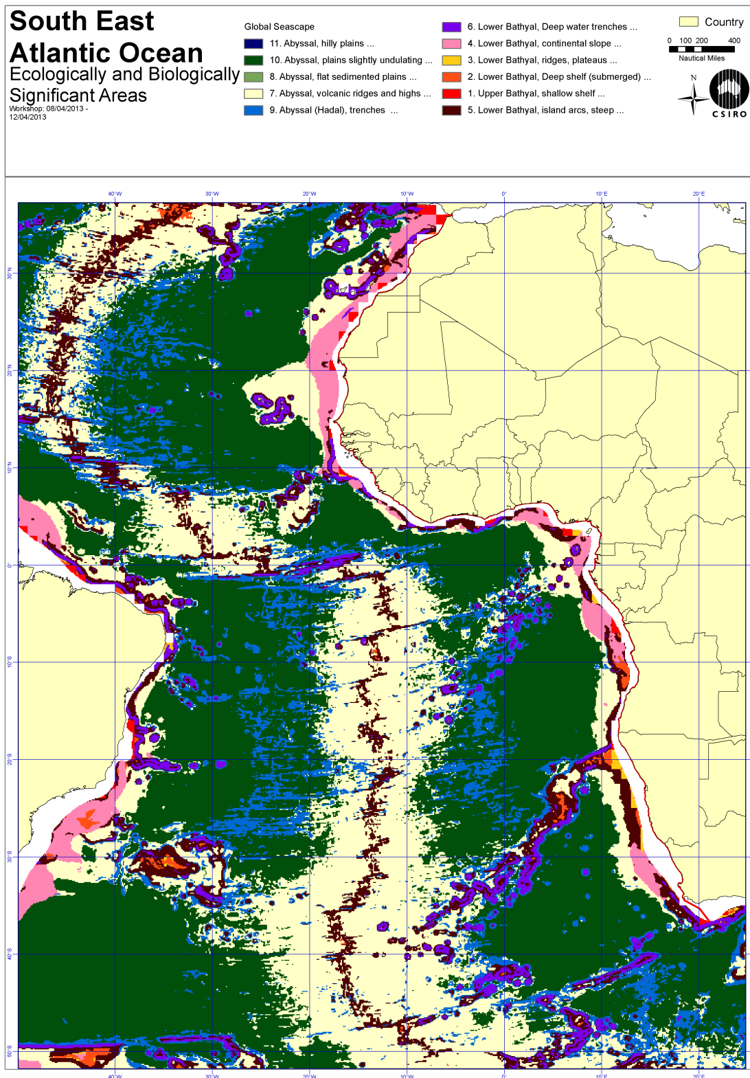
Figure 4.2: Derived Global Seascapes
