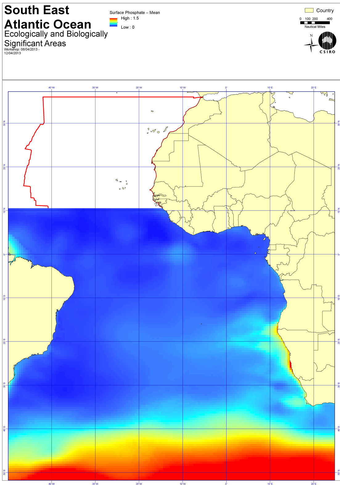
Figure 4.15: Annual Phosphate
