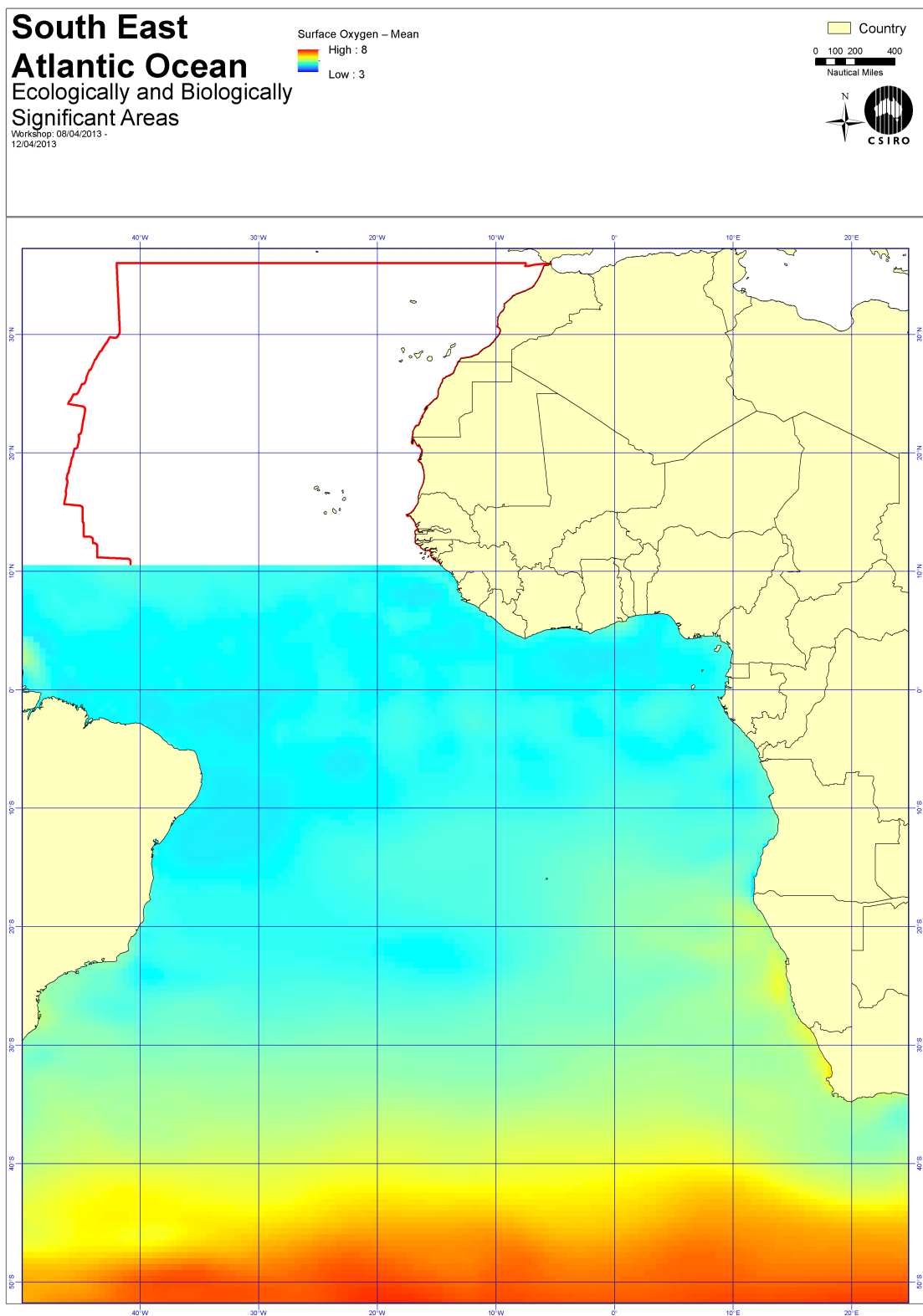
Figure 4.12: Annual Oxygen
