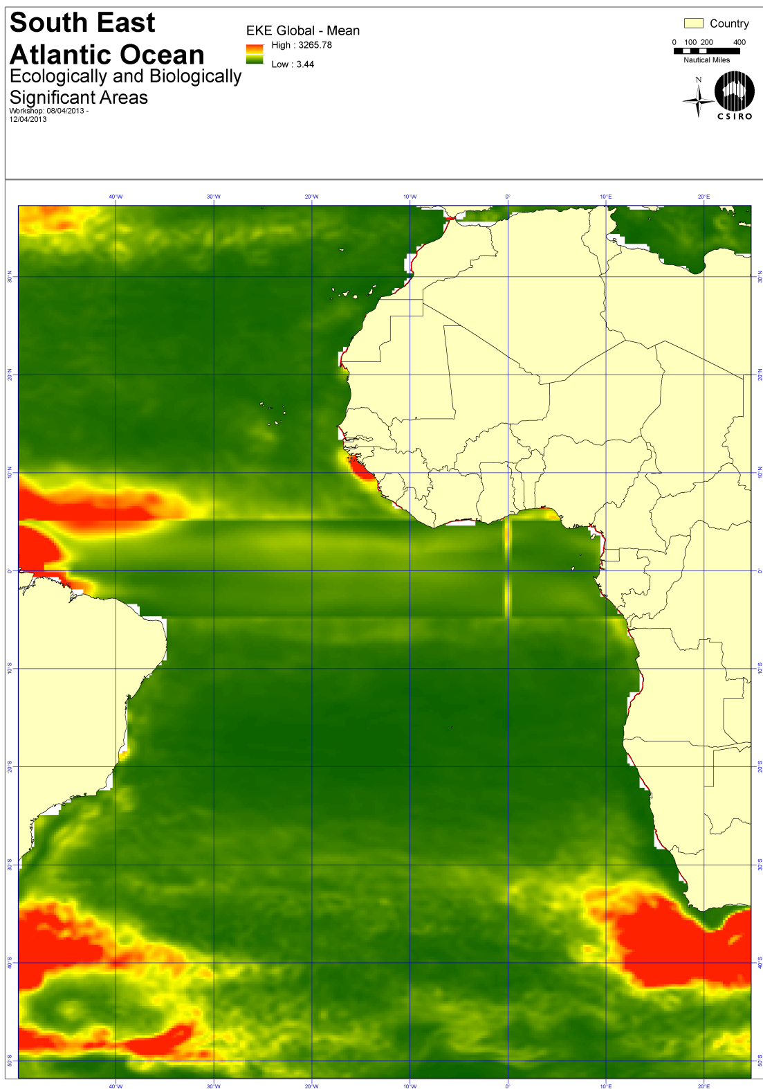
Figure 4.21: Annual Eddy Kinetic Energy
