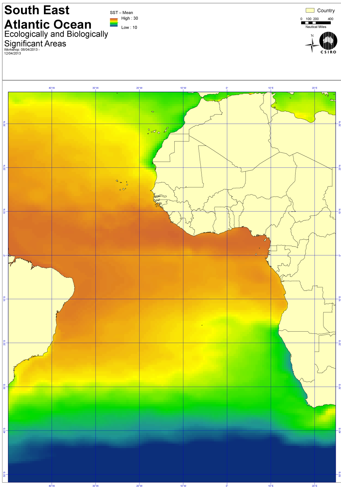
Figure 4.10: Annual SST
