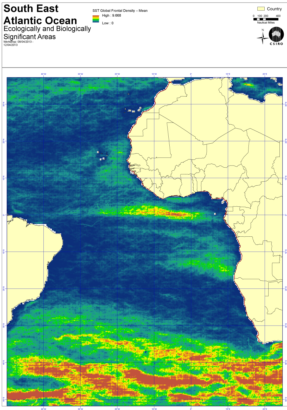
Figure 4.20:
