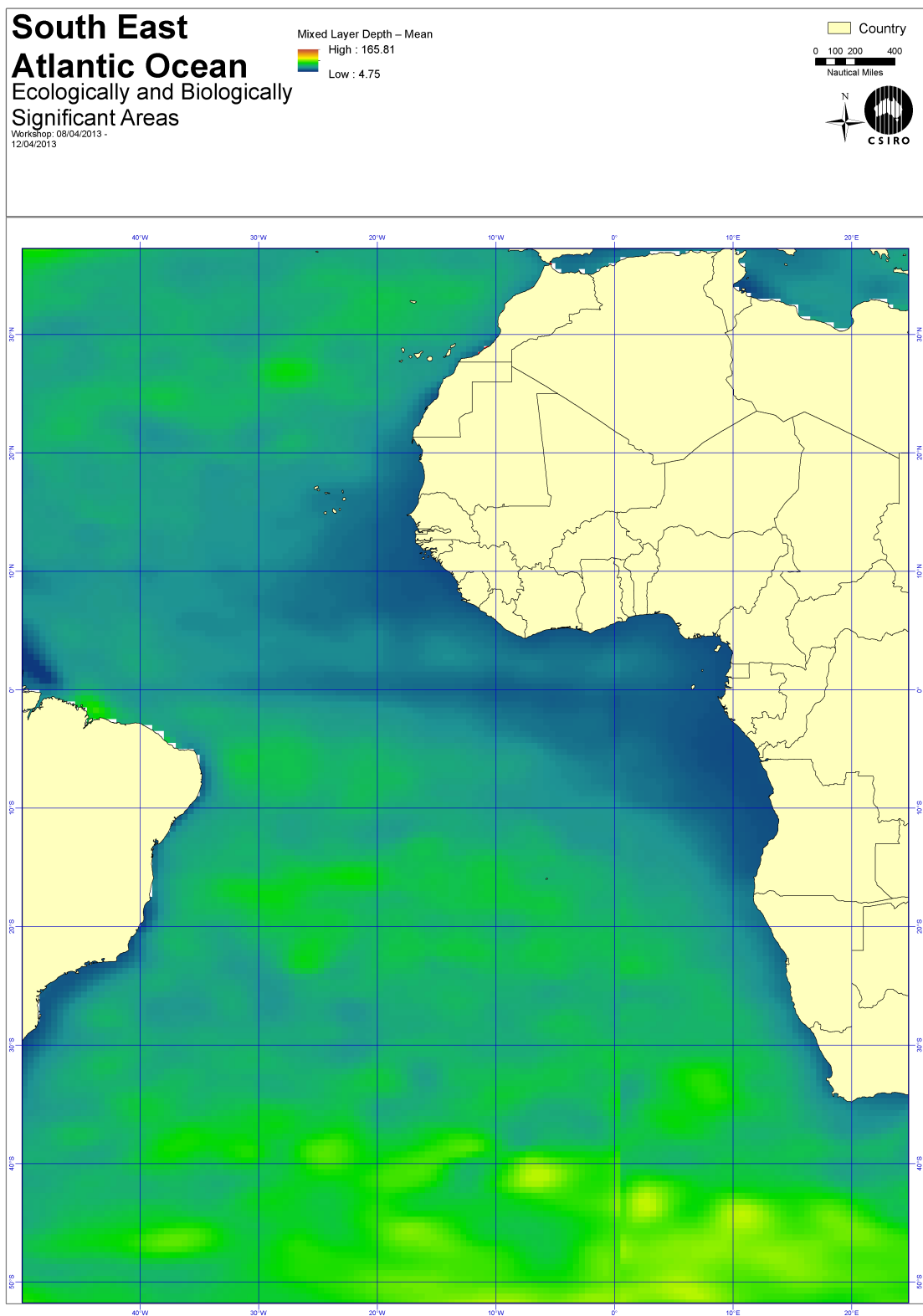
Figure 4.19: Annual Mixed Layer Depth
