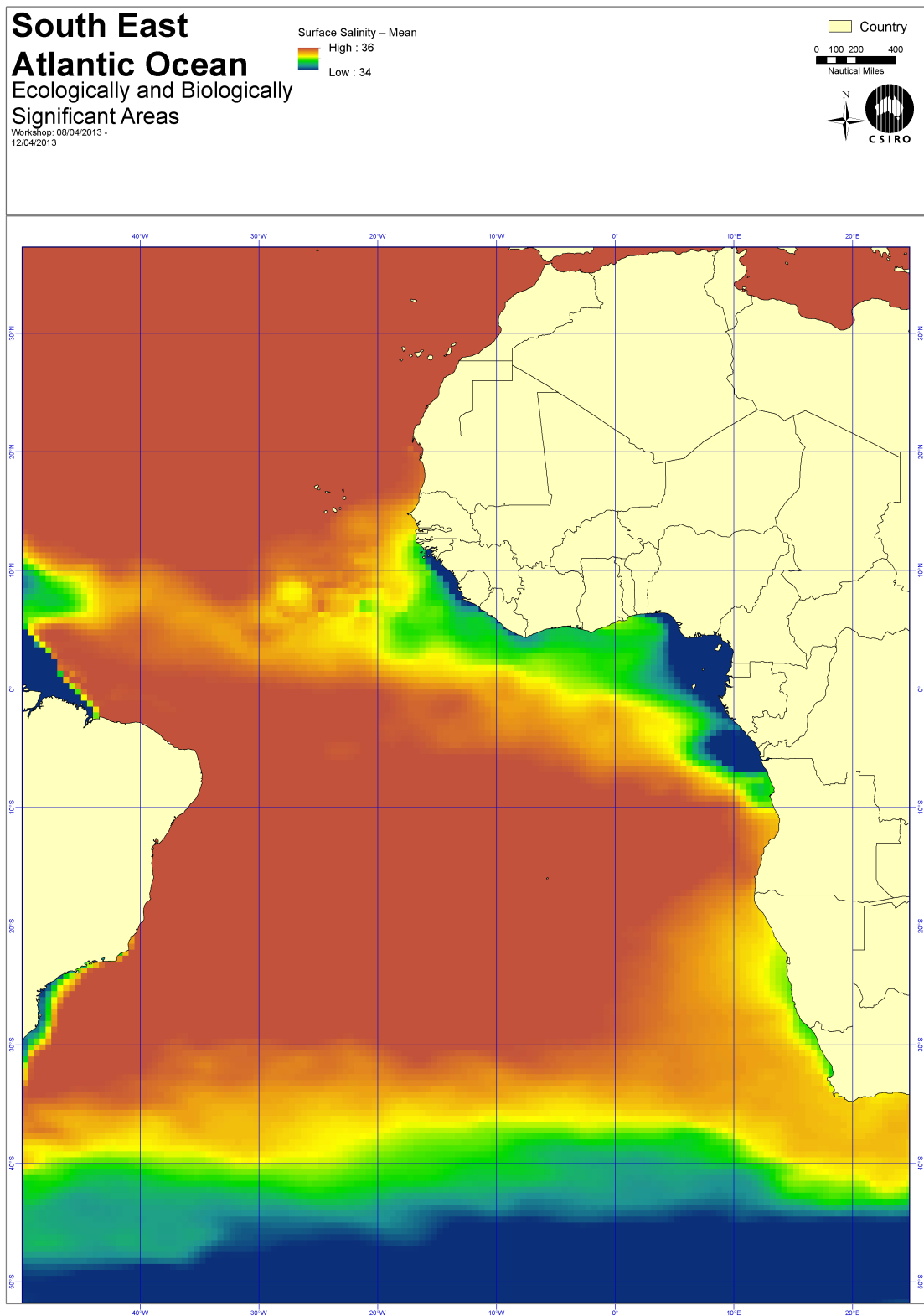
Figure 4.11: Annual Salinity
