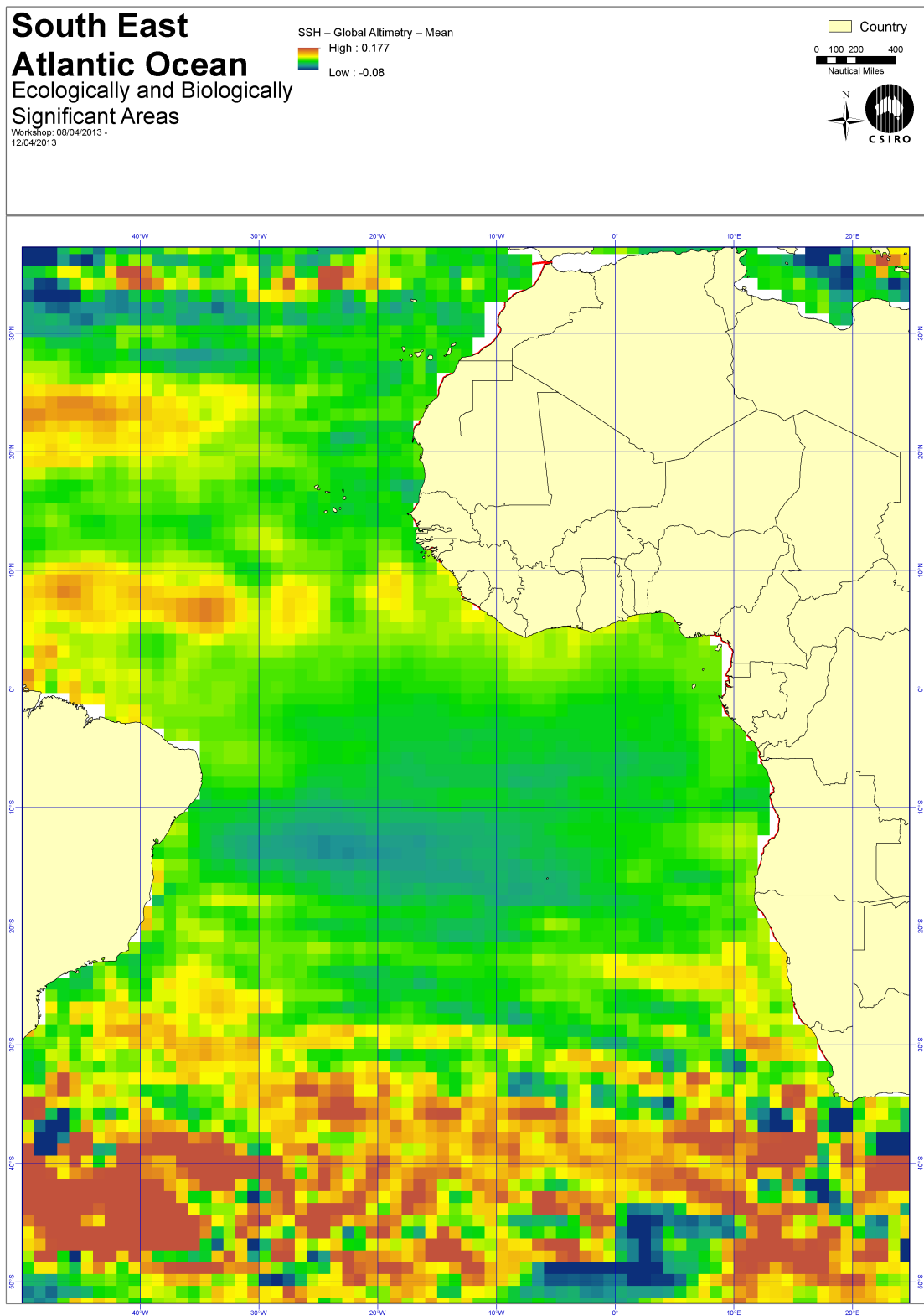
Figure 4.16: Annual sea surface height
