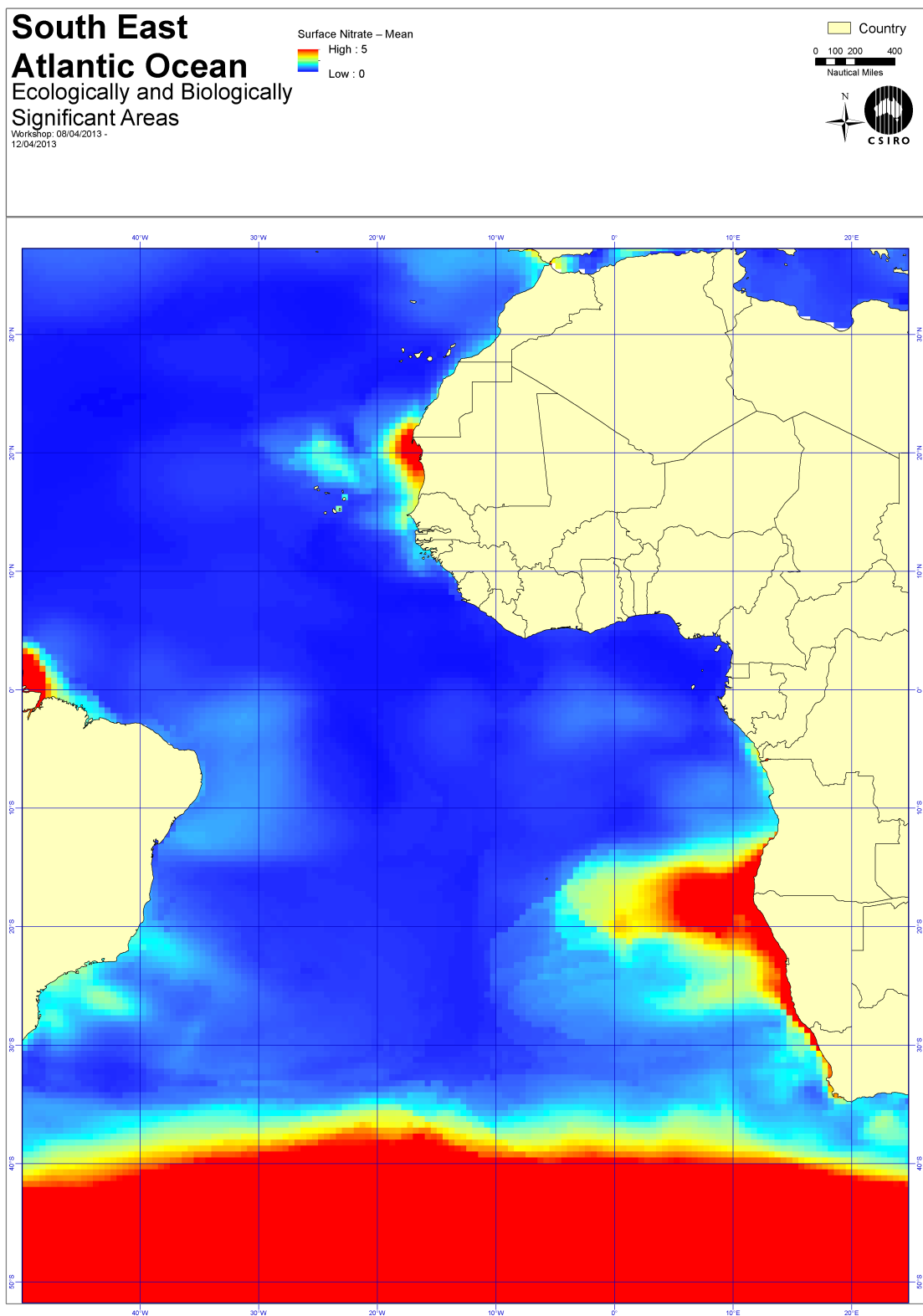
Figure 4.13: Annual Nitrate
