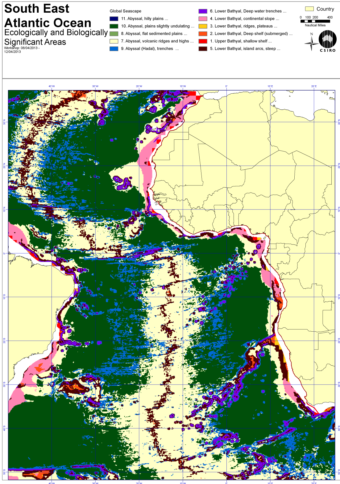
Figure 4.2: Derived Global Seascapes
