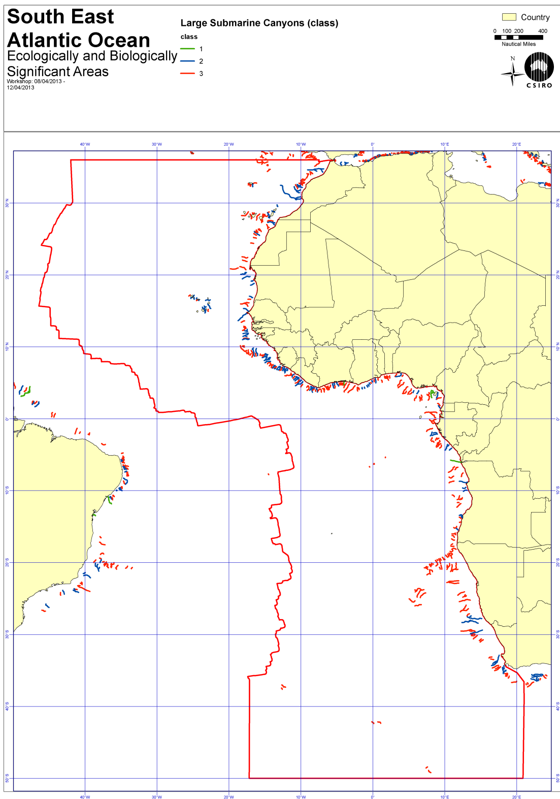
Figure 4.8: Large Submarine Canyons
