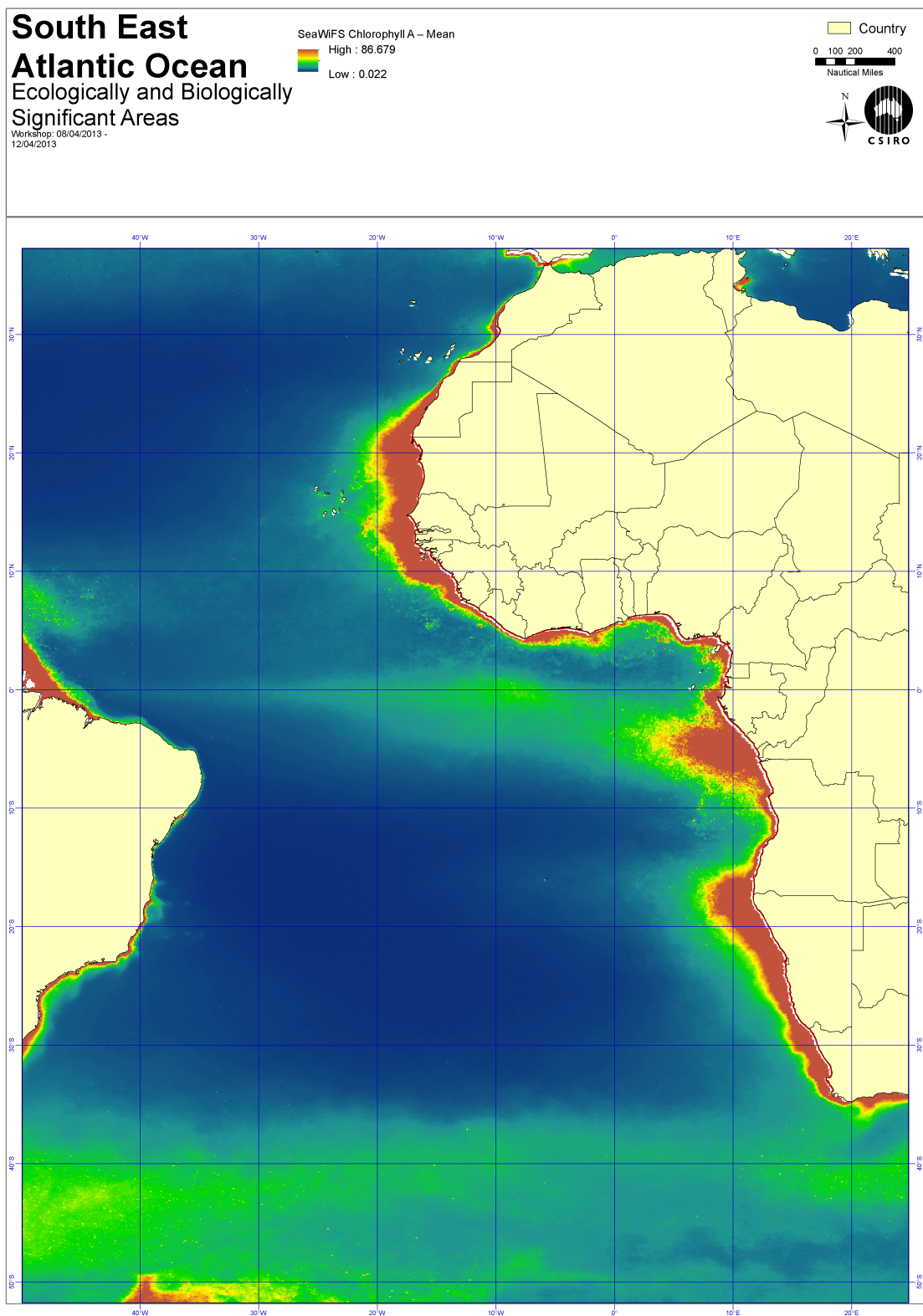
Figure 4.17:
