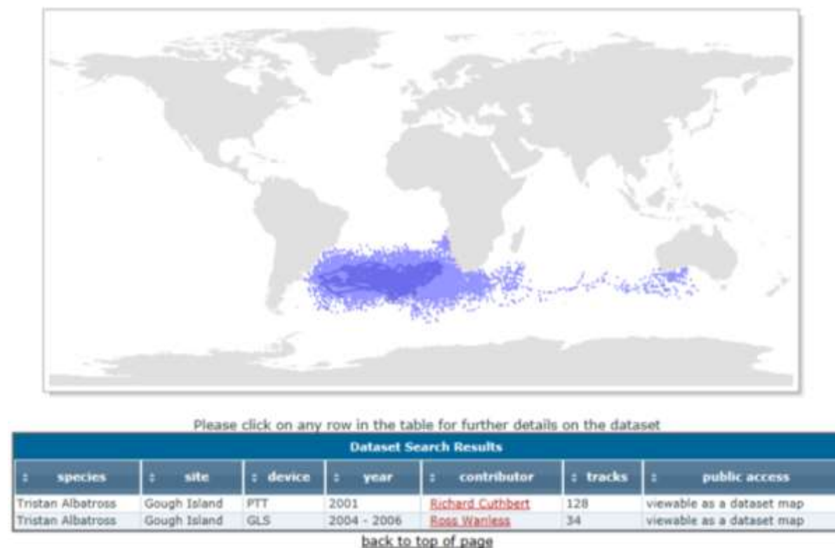
Figure 1. Overall extent of tracking data for Tristan Albatross held at www.seabirdtracking.org .
