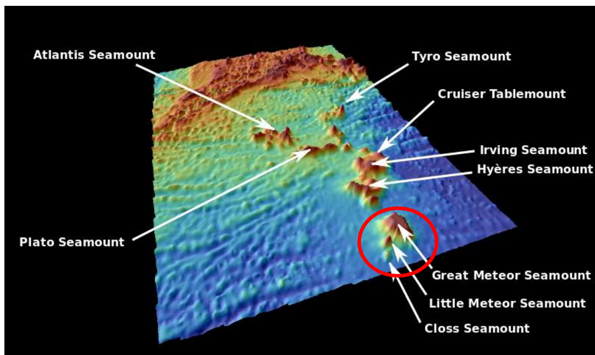
Figure 1. The Seewarte Seamounts and the Azores bulge to the north.
