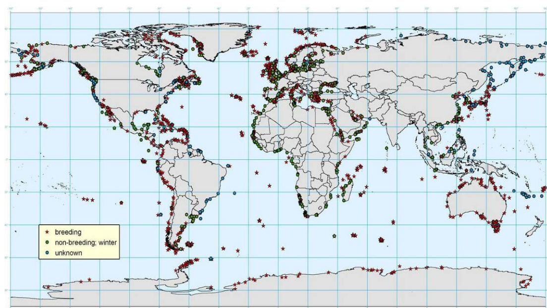
Figure 2: Map of candidate marine IBAs, showing sites qualifying during the breeding and non-breeding seasons. Data correct to August 2008
