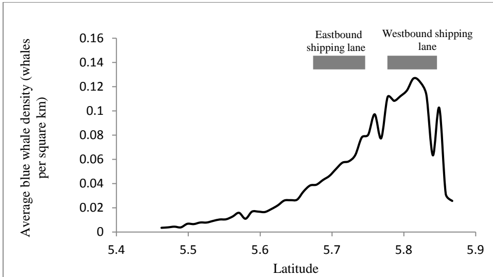
Figure 7. Average modelled blue whale density by latitude between longitudes 80^{\circ} 25' and 80^{\circ} 45' . Latitudes of eastbound and westbound shipping lanes off Dondra Head shown as grey bars.
