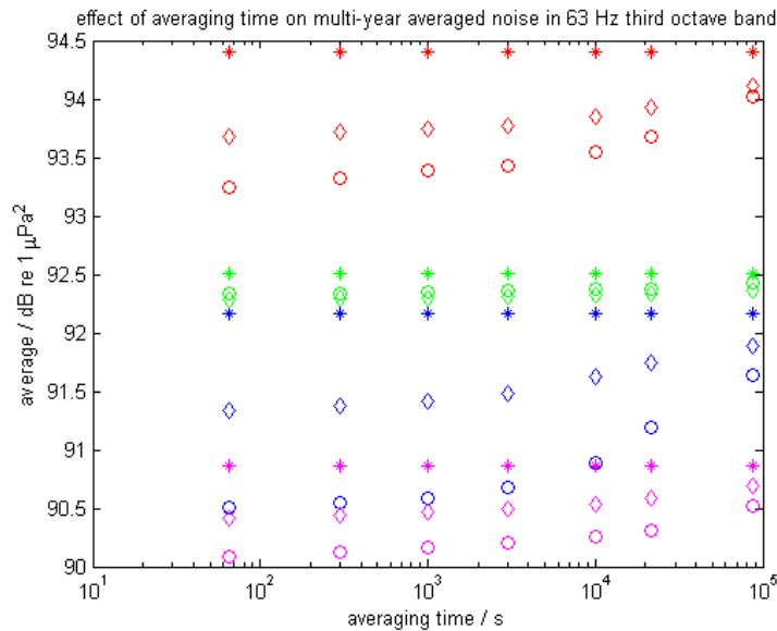
Figure 32: Arithmetic mean (asterisks), geometric mean (diamonds) and median (circles) plotted vs snapshot duration for four CTBTO sites; colours: A scension I sland, C ape L eeuwin, W ake I sland, J uan F ernández. The averaging times (snapshot durations) are 65 s, 300 s, 1000 s, 3000 s, 10000 s, 21600 s and 86400 s.
