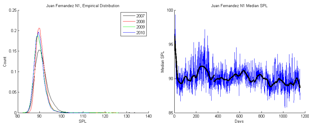
Figure 26: Left graph: Histogram of SPL 63 distribution for Juan Fernández Islands ( T = 65.5 s); daily median of SPL 63 vs time.
