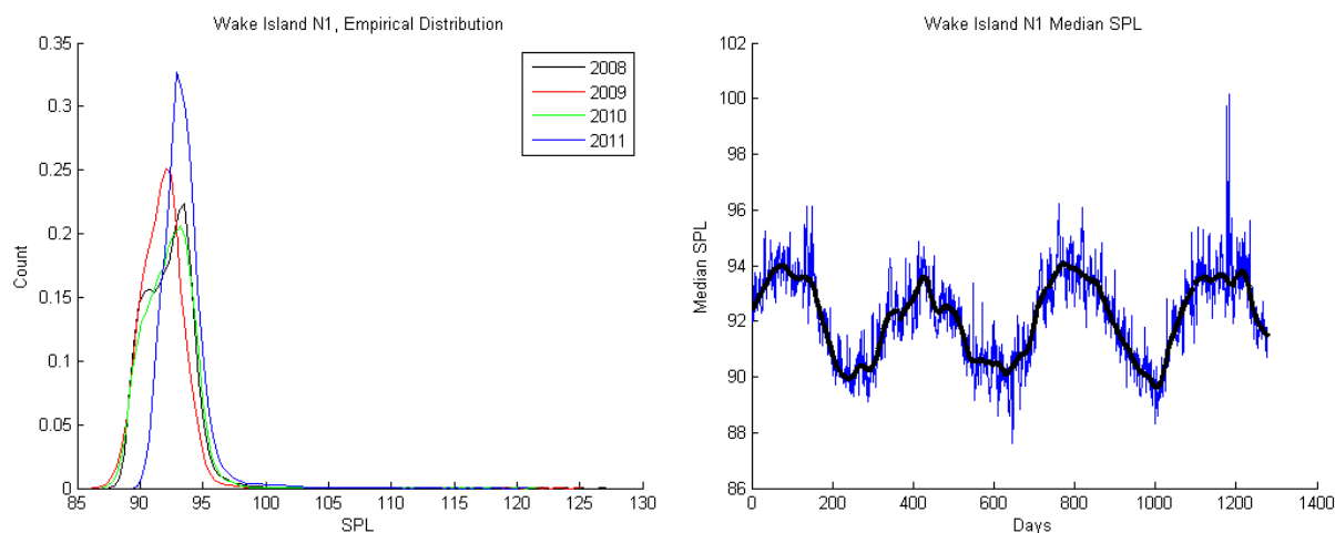
Figure 28: Left graph: Histogram of SPL 63 distribution for Wake Island ( T = 65.5 s); daily median of SPL 63 vs time.
