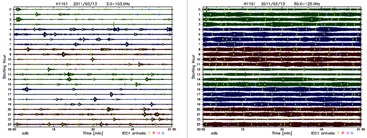
Figure 31: Pressure time series (24 h) for Wake Island on 13 March 2011. Left: broadband (3 Hz to 103 Hz); right: filtered in the frequency band 50 Hz to 125 Hz.
