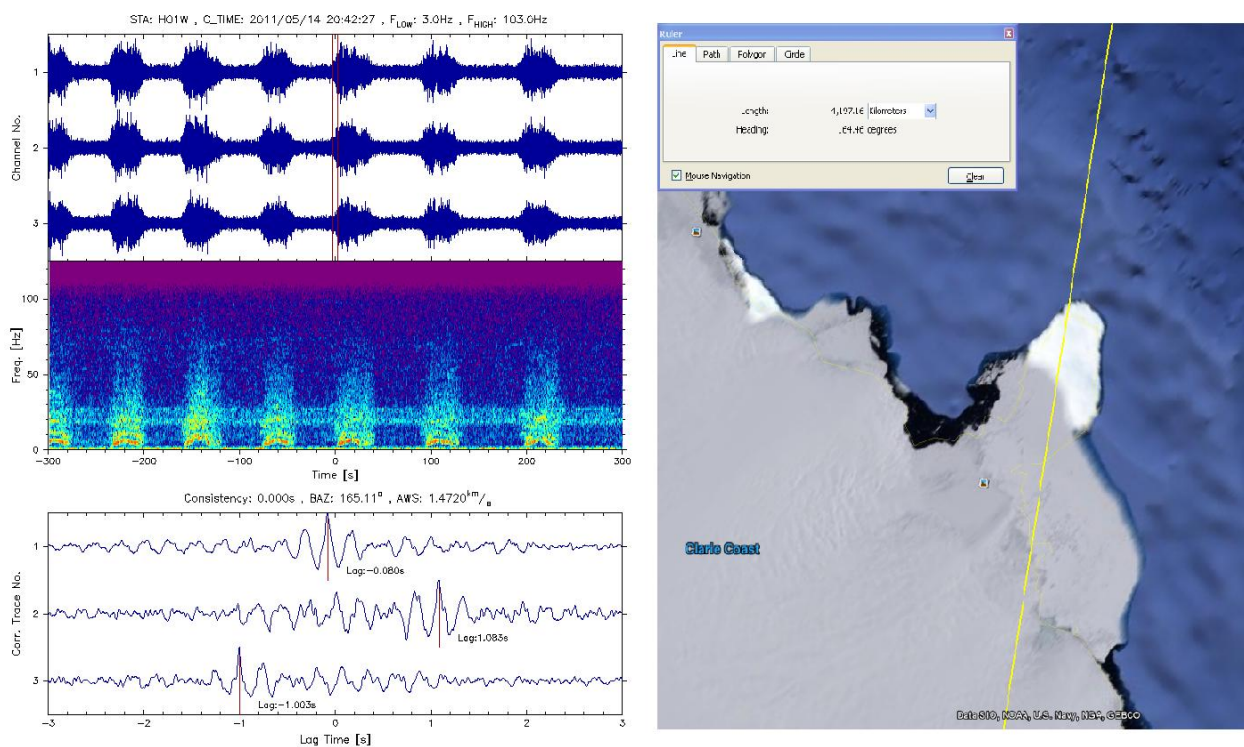
Figure 24: Left: Close-up of broadband (3 Hz to 103 Hz) pressure time series and spectrogram at 20:42:27 \pm 300 s on 14 May 2011 for Cape Leeuwin; lower graph shows time lag plot indicating sound originates from bearing 165 deg. Right: Ice tongue on Antarctica at bearing 165.
