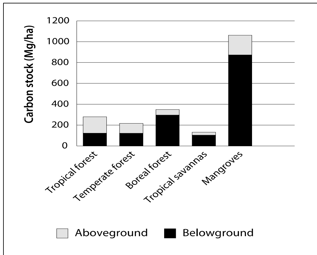
Figure 9: Total ecosystem carbon pools for some major land cover types
