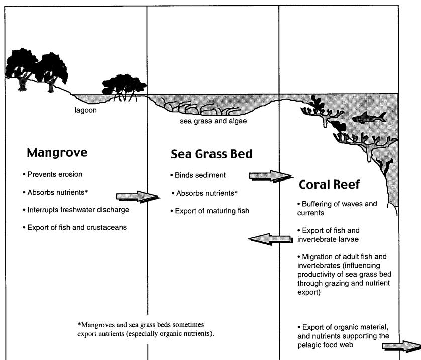
Figure 10: Interactions in the tropical seascape, showing the connections between mangroves, seagrass beds and coral reefs
