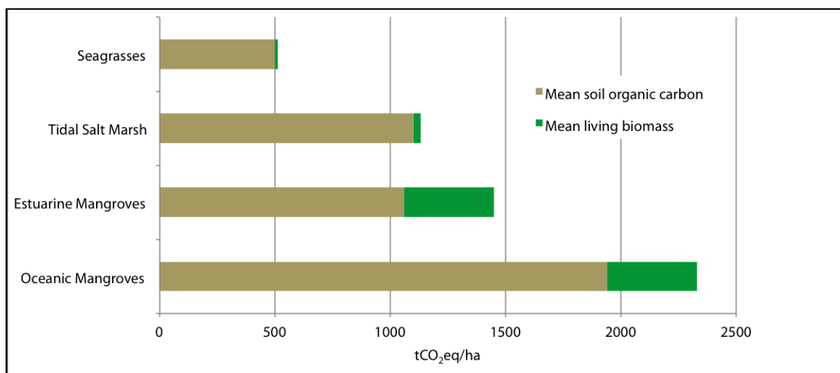
Figure 8: Global averages of above- and below-ground carbon pools of marine and coastal ecosystems
