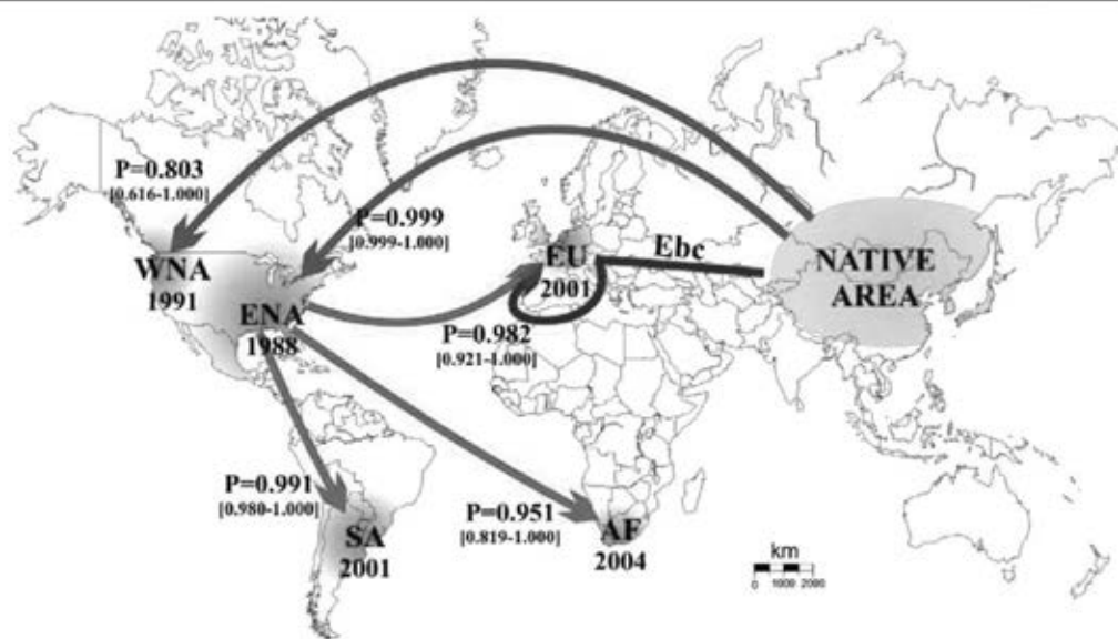
Figure IX.1 Spread of Harmonia axyridis (Lombaert et al. 2010)
