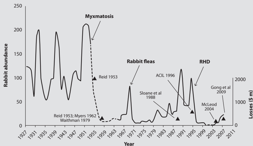
Figure V.1. Diagram showing how rabbit abundance in semi-arid South Australia has varied through time in response to the release of biocontrol agents. The estimated Australia-wide economic losses to rabbits (black triangles) are also shown. Scale for losses shown on right-hand side of figure. Figure adapted from Saunders et al. (2010)
