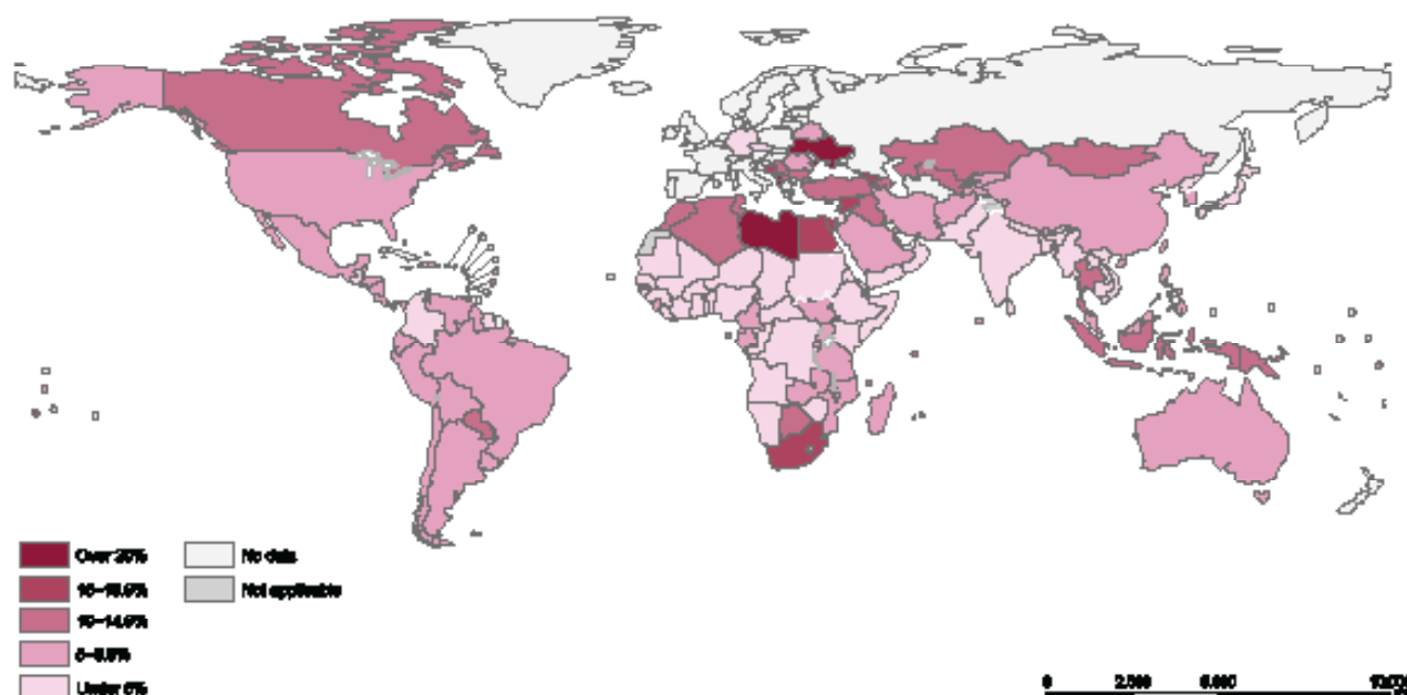
Percentage of children age 0–59 months who are overweight
