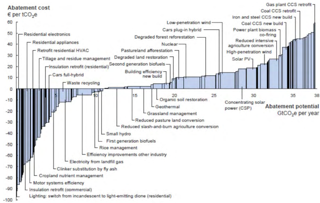
Figure 1.2: Global GHG abatement cost curve beyond business-as-usual 2030
