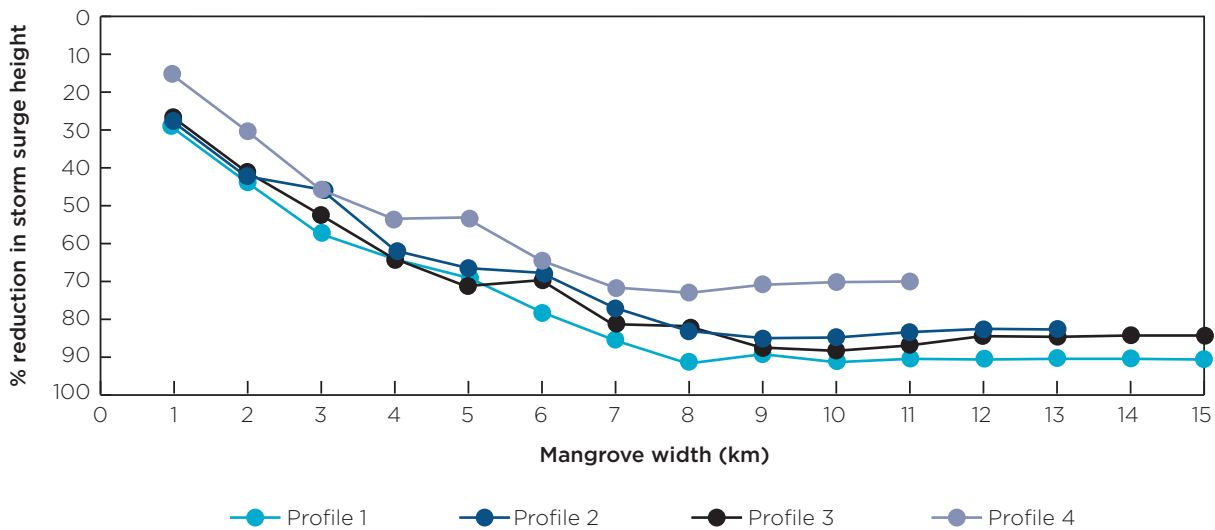
Figure 2.7: Reduction of Storm Surge Height by Mangroves on the Gulf Coast of South Florida, United States during Hurricane Wilma (2005, Category 3 on impact), Modeled using CEST (data from Zhang et al. 2012)
