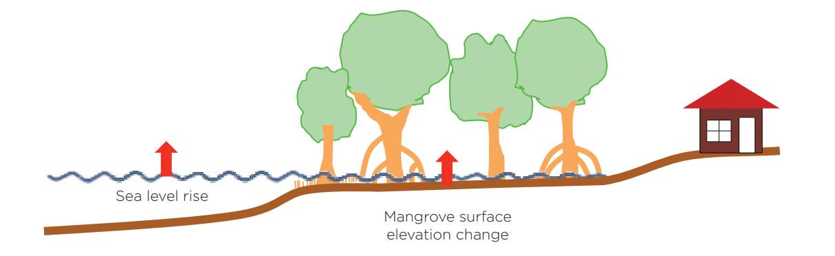
Figure 2.8: Diagram Showing how Mangrove Soil Surfaces can Rise with Sea-level Rise, Potentially Allowing Mangroves to Keep Pace with Sea-level Rise
