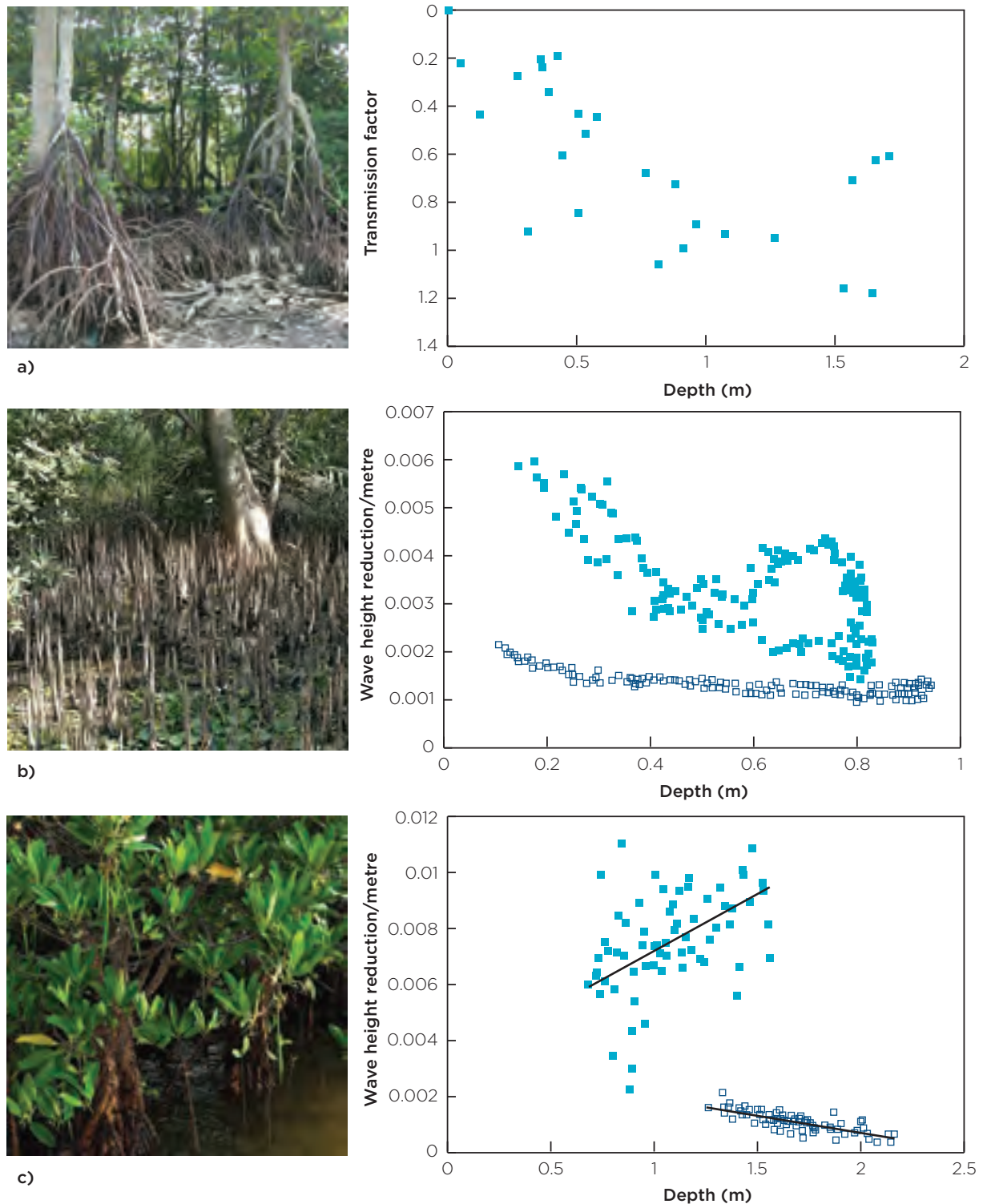
Figure 2.3: Wave Attenuation through Three Mangrove Species
