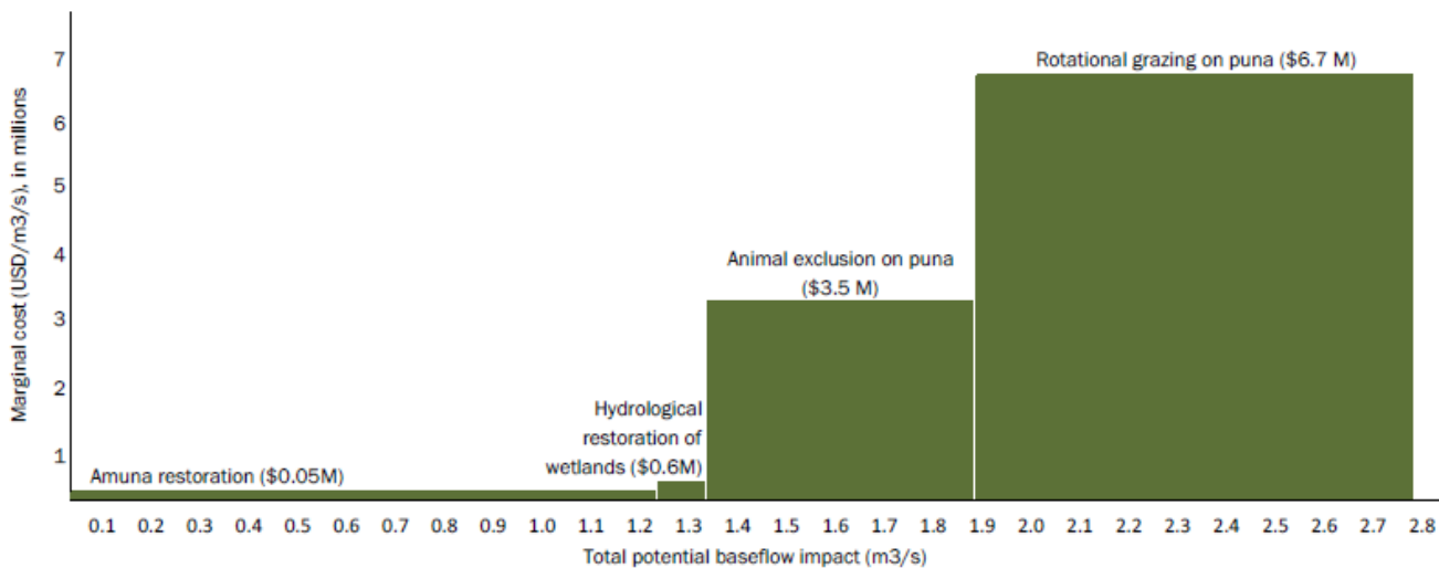
Figure 2. Cost curve of green interventions for improving dry season water supply for Lima.
