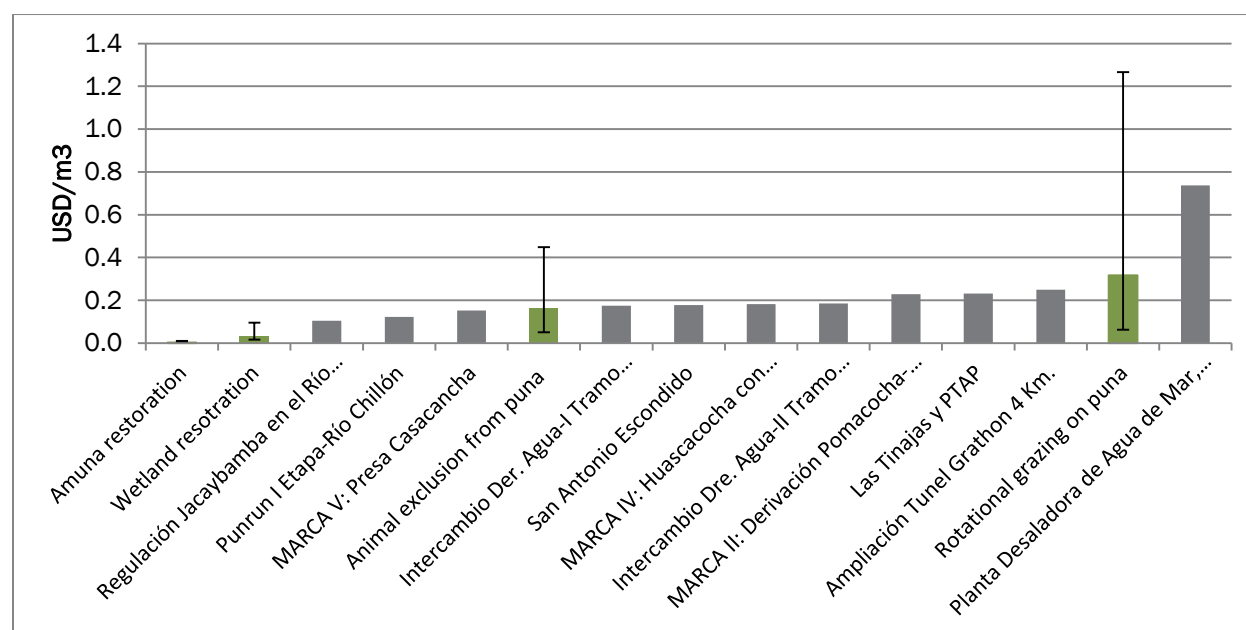
Figure 4. Costs (USD/m 3 ) of green and gray interventions for Lima's water supply. Sources: current analysis and Nippon Koei (2011).
