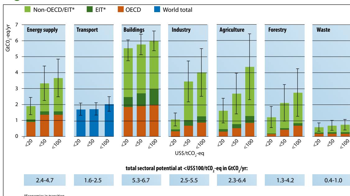
Figure 8. IPCC projections of CO 2 mitigation potential in 2030.
