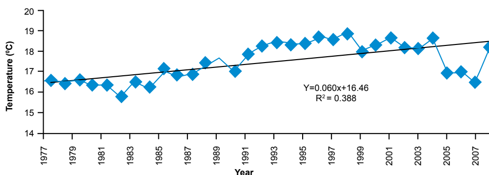
Figure 10: Annual average temperature in CDR
