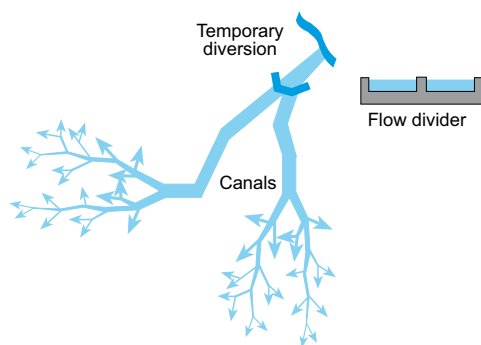
Tara Prasad Bhond: Locally made divider, 16-36 Mauja irrigation system
