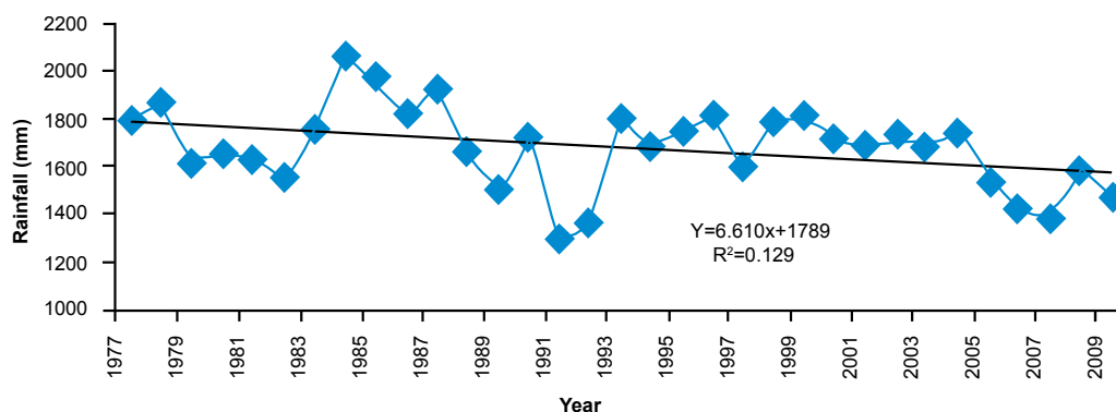
Figure 12: Average annual rainfall in CDR
