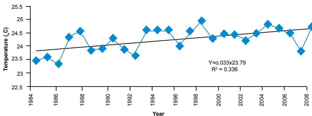
Figure 9: Annual average temperature
