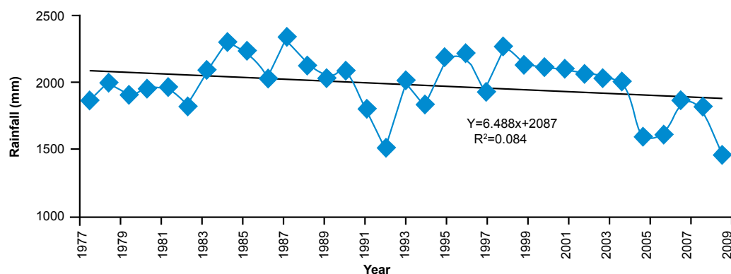
Figure 11: Annual average rainfall in the midhill districts
