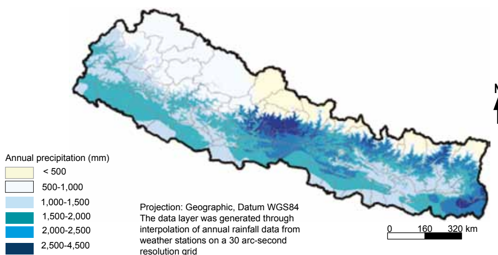
Figure 2: Annual precipitation map of Nepal
