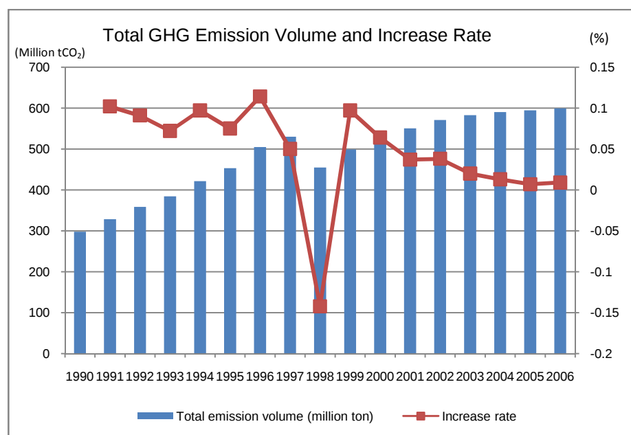
Figure 3. Annual total GHG emission volume and increase rate, 1990-2006
