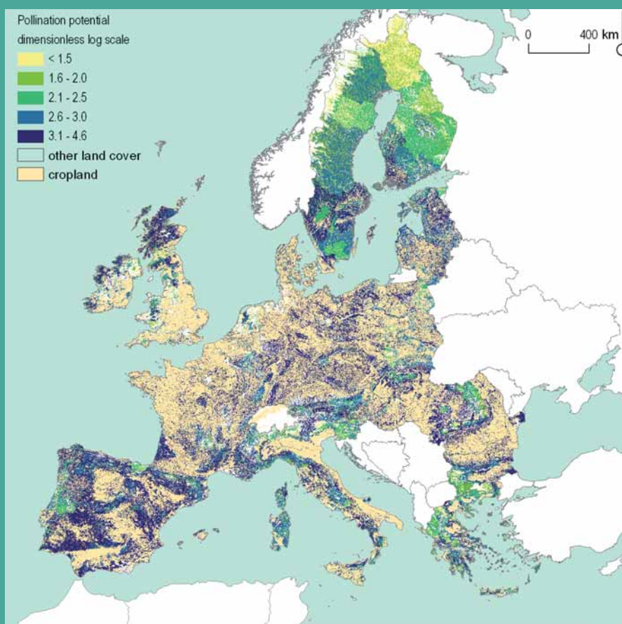
Figure 7: Pollination potential, 1km resolution
