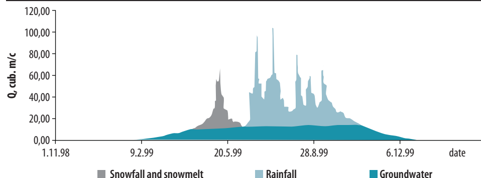
Figure 30: Runoff components in Tuul River flow at Ulaanbaatar
