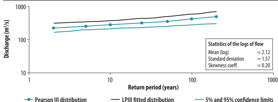
Figure 31: Flood frequency analysis for the Tuul River at Zaisan
