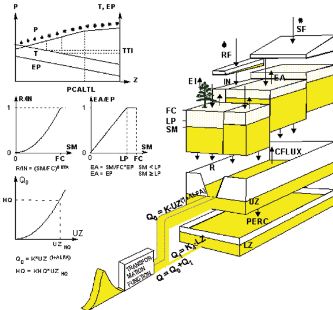
Figure A.1. Schematic structure of one sub-basin in the HBV-96 model 72 , with routines for snow (top), soil (middle) and response (bottom)
