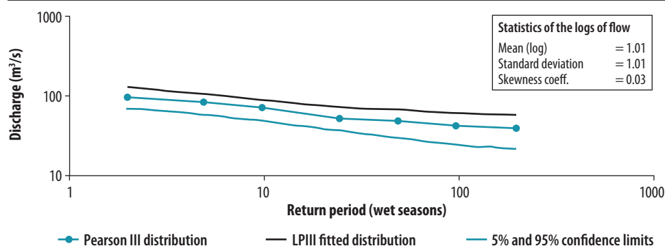
Figure 32: Low flow frequency analysis for the Tuul River at Zaisan
