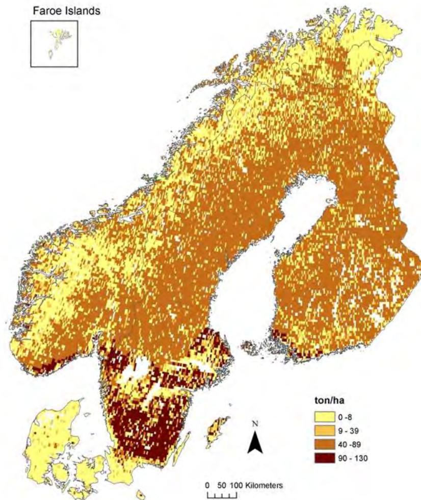
Figure 9.2 Carbon storage (above and below ground) in the Nordic countries (tonnes / ha) based on the models of JRC. (Maes et al. 2011a, 2011b)
