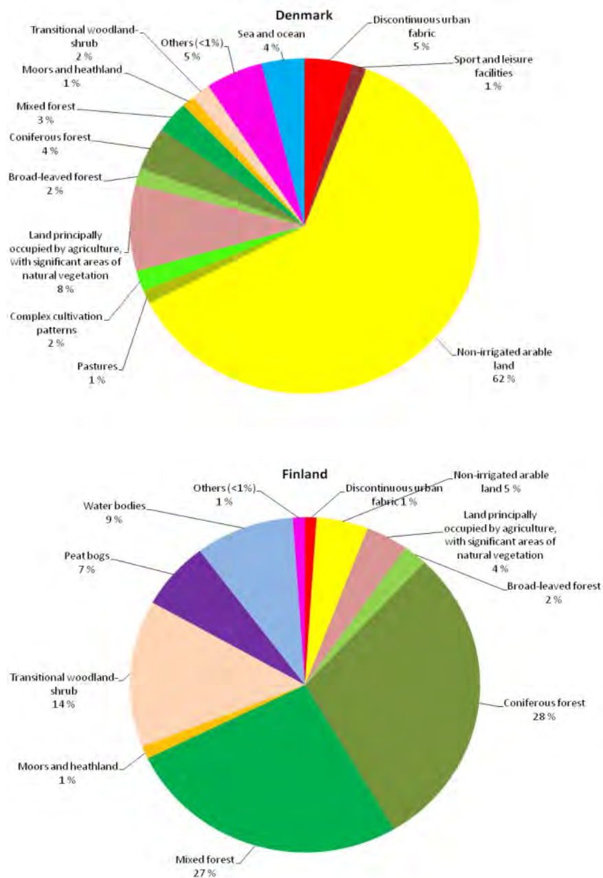
Figure 7.3 a-e: Main land cover types of the Nordic countries. The classes of which share of the total land cover were less than 1% are summed together to the class “others”
