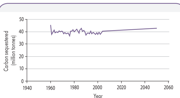
Figure 22.4 Estimated carbon sequestration by marine phytoplankton in UK shelf seas, 1961–2050.*
