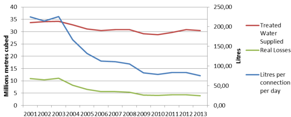
Figure 10 Leakage reduction in Malta
